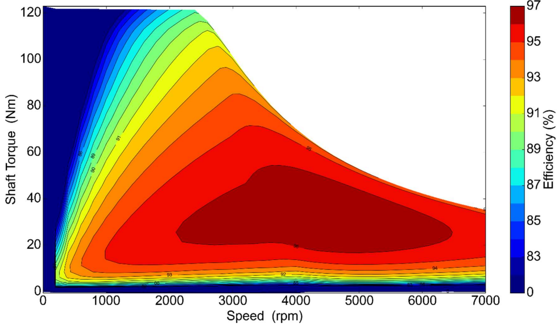
Efficiency Map % (*)
